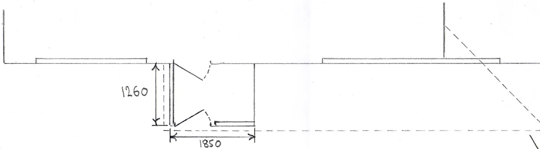
EXISTING PLAN
